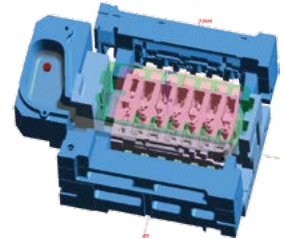
Detailed process model with mold halves, slides, sand cores or inserts, as well as complex cooling and heating lines.
