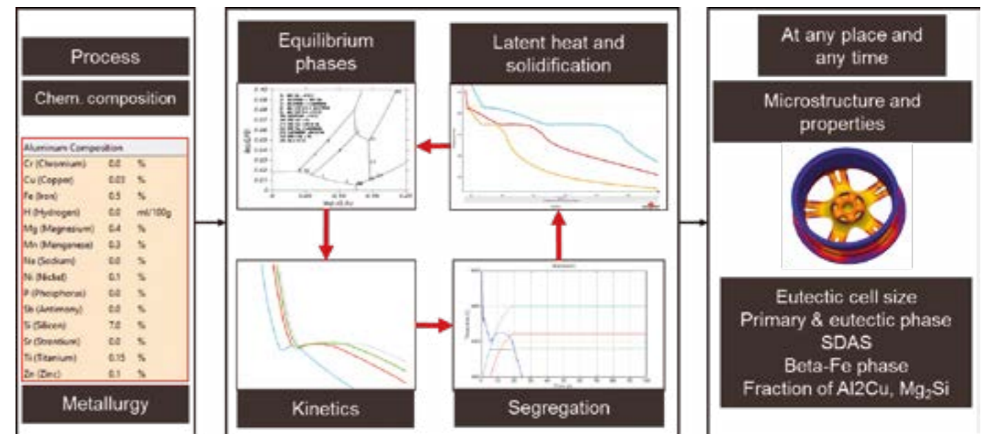
Calculation loop for prediction of local microstructure and resulting mechanical properties
