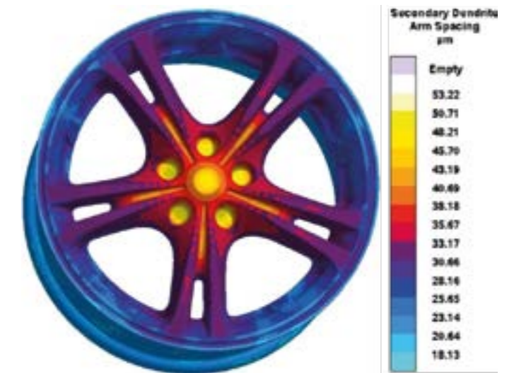
Calculated local secondary dendrite arm spacing
