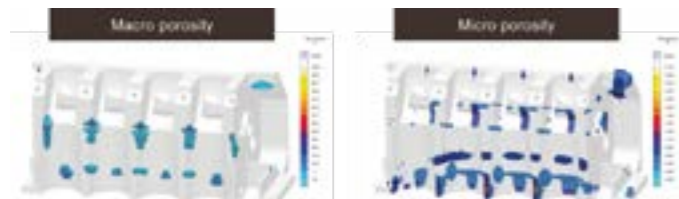
Display of macro- and microporosity
