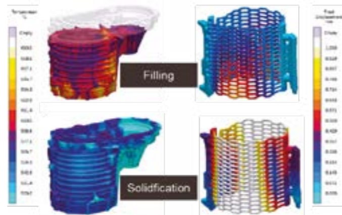
Deformation of sand cores during mold filling and solidification
