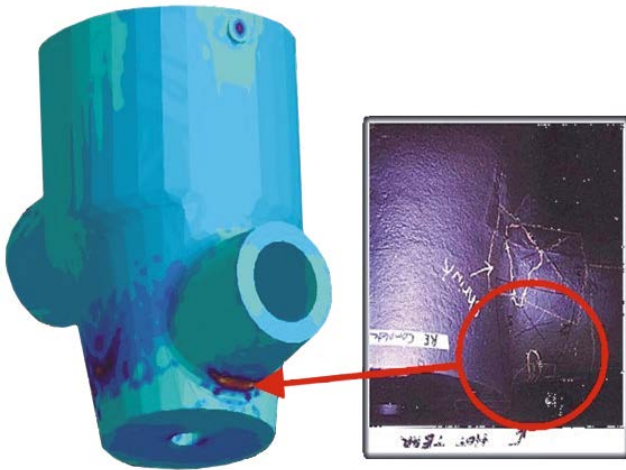
Hot tear: prediction and real defects
