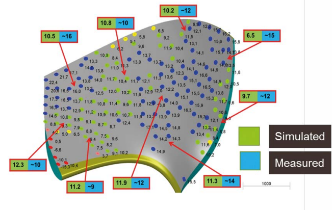
Comparison of measured and calculated distortions
