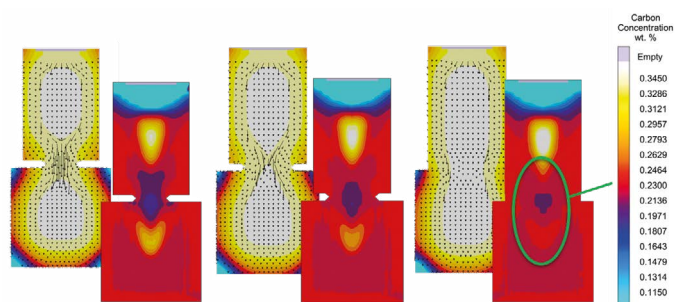
Predicting under-riser segregation
